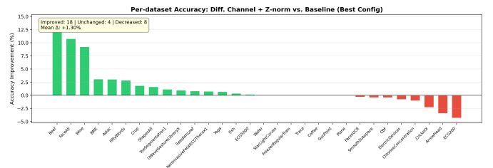
Fig. 2. Dataset-level improvement comparison demonstrating performance gains from optimization strategies including AdamW and differenced input channels.
