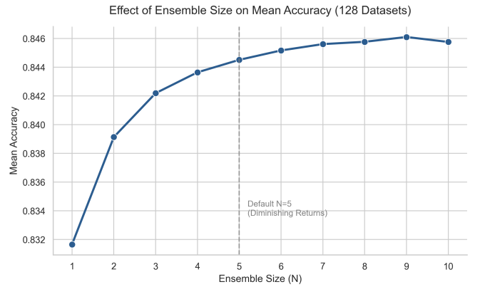
Fig. 6. Effect of ensemble size on classification accuracy. Performance improves with increasing ensemble size before stabilizing.
