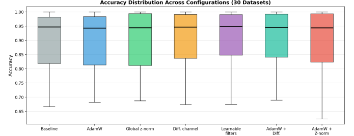
Fig. 5. Accuracy distribution across univariate datasets demonstrating performance consistency across configurations.
